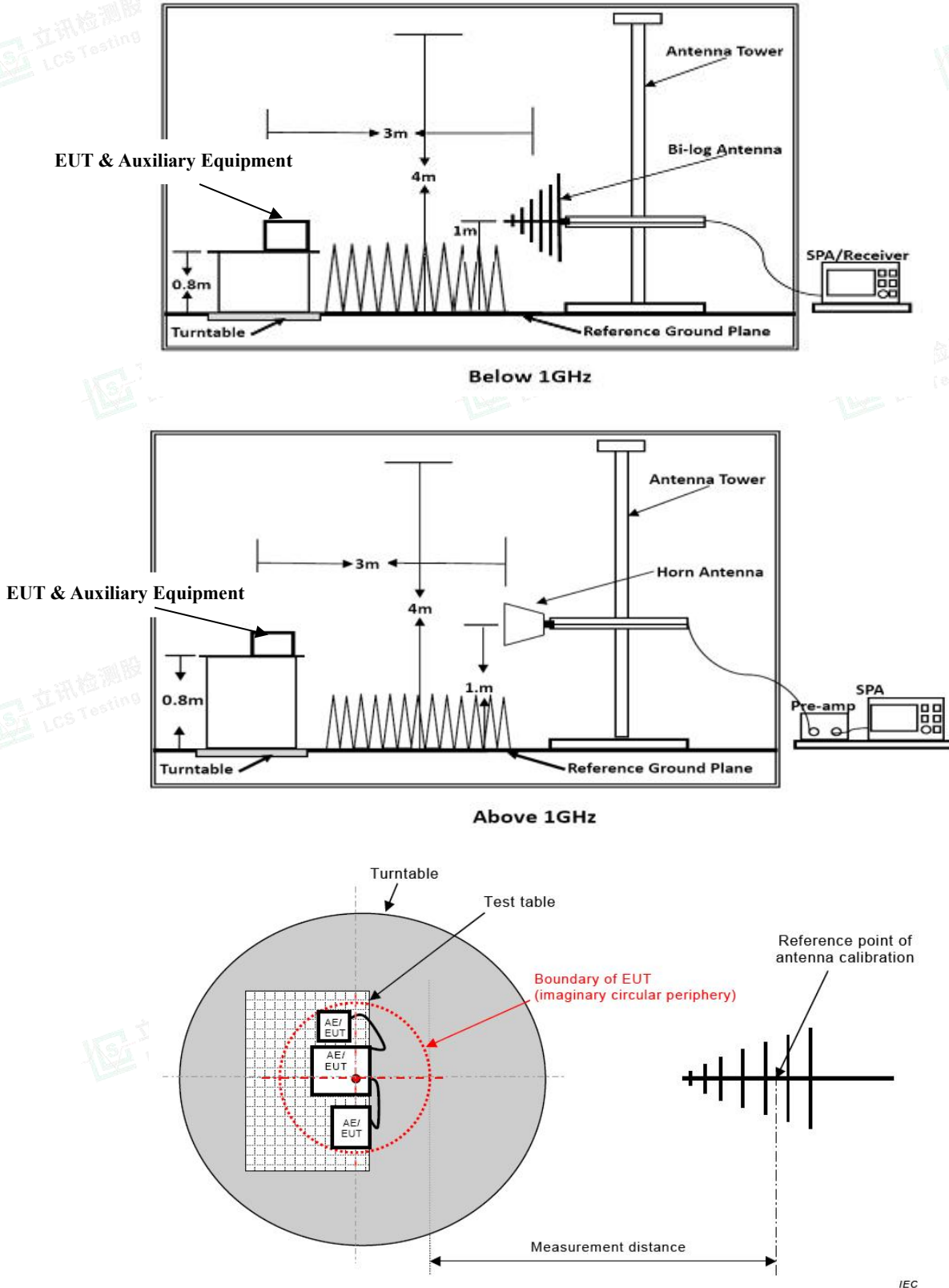
Figure C.1 – Measurement distance
